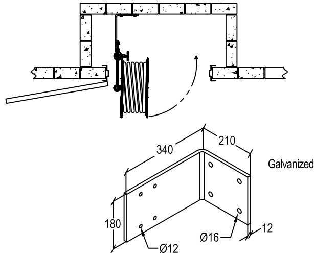
STAND OFF BRACKET for PROTRUDING ARCHITRAVE
